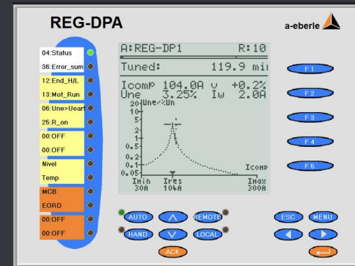
Regulator automat A-EBERLE tip REG-DPA
