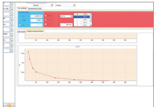
PADS SOFTWARE
