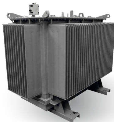
Fig. 1 TKFC 3-phase shunt reactor – 500 kVA - corrugated tank – hermetically sealed
